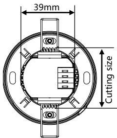
Figure 4. Dimensions - Back View
