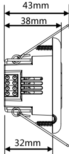
Figure 3. Dimensions - Side View
