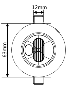
Figure 2. Dimensions - Front View
